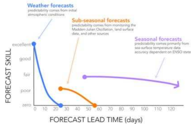
FIGURE 8: FORECAST SKILL AT INCREASING LEAD TIMES. SKILL IN WEATHER PREDICTION IS HIGH AT LEAD TIMES OF A FEW DAYS, BUT DECREASES SHARPLY BEYOND THIS
